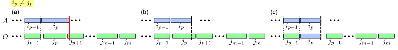
Figure 2: The case when i_p \neq j_p , for some p > 1 . We show only the jobs i_{p-1} and i_p in A . Black dots indicate earlier, intermediate, or later jobs. (a) Can the finish time of i_p be larger than the finish time of j_p (potentially causing i_p and j_{p+1} to conflict)? (b) No! The reason is that both i_p and j_p start after i_{p-1} finishes. Therefore, after the EFT algorithm has selected i_{p-1} and included it in A , both i_p and j_p (which are compatible with i_{p-1} ) were available for being chosen as the next job in A . However, the EFT algorithm selected the job i_p . Hence, its finish time must be less than or equal to the finish time of j_p . (c) Therefore, if we replace j_p with i_p in O , all the jobs in O continue to be mutually compatible.
