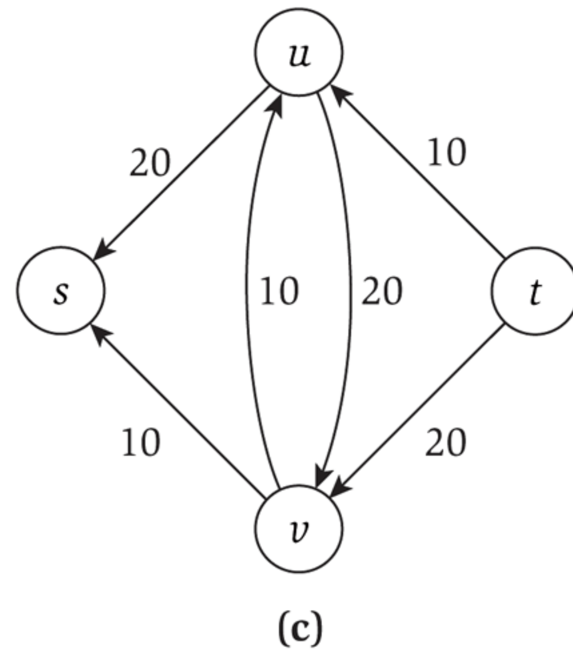
Figure 7.4 (a) The graph G with the path s, u, v, t used to push the first 20 units of flow. (b) The residual graph of the resulting flow f , with the residual capacity next to each edge. The dotted line is the new augmenting path. (c) The residual graph after pushing an additional 10 units of flow along the new augmenting path s, v, u, t .
