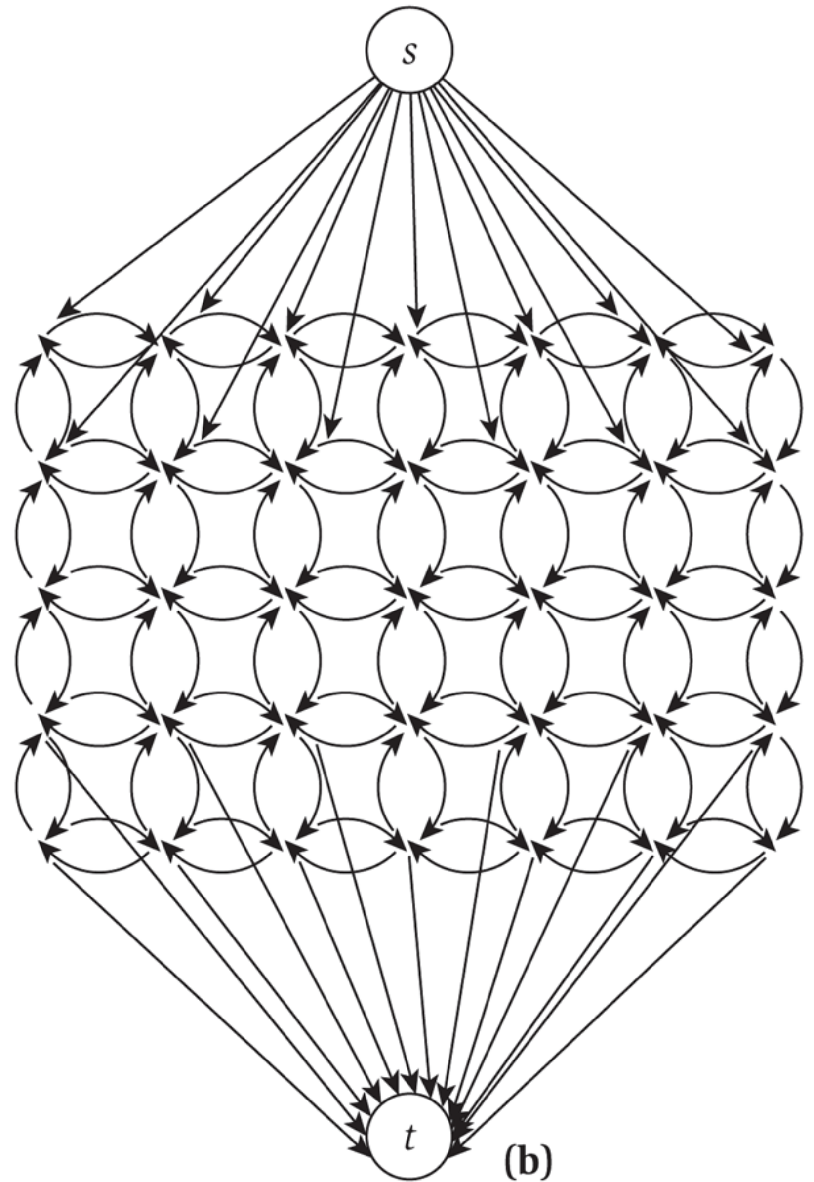
Figure 7.18 (a) A pixel graph. (b) A sketch of the corresponding flow graph. Not all edges from the source or to the sink are drawn.
