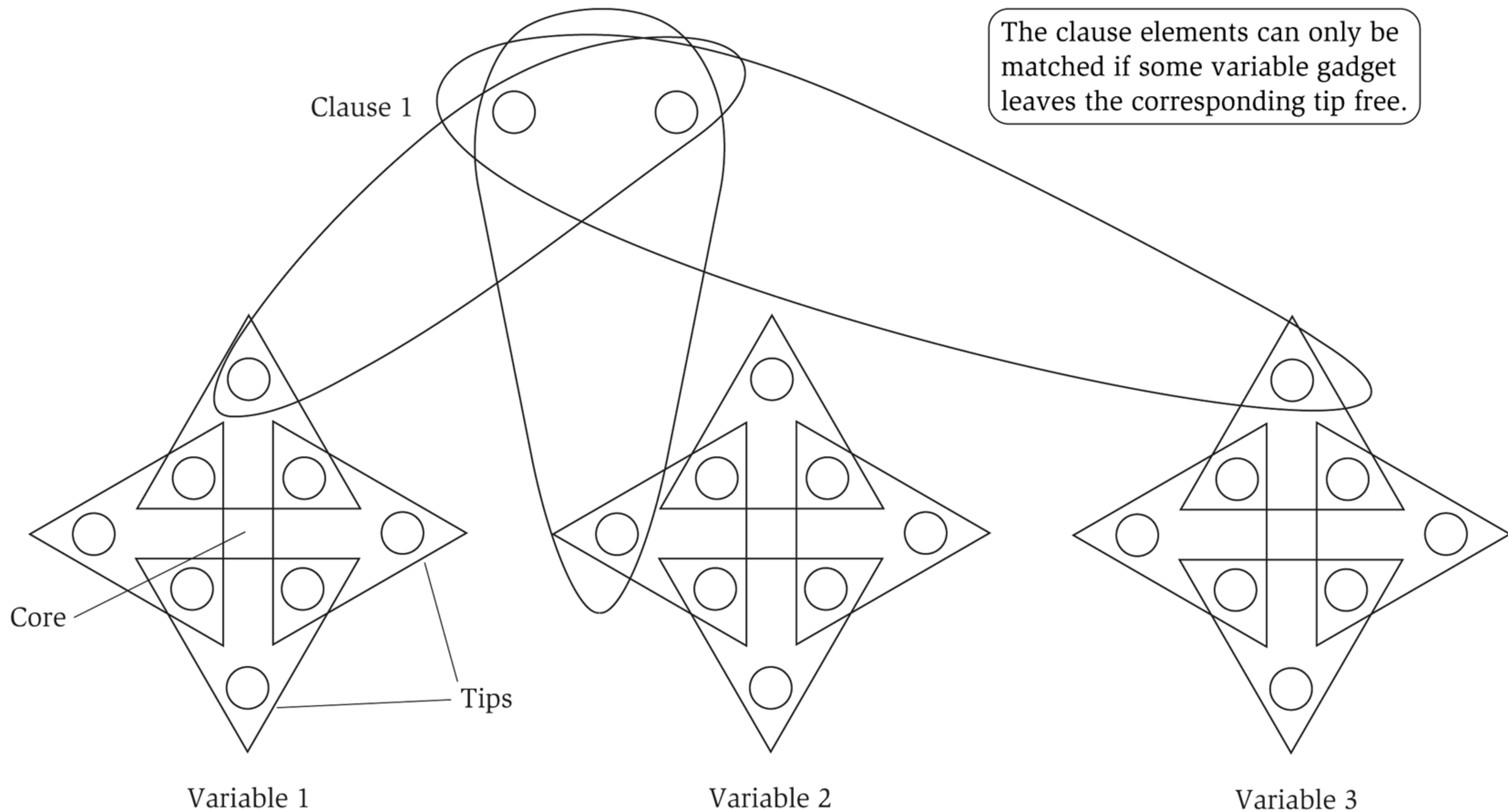
Figure 8.9 The reduction from 3-SAT to 3-Dimensional Matching.
