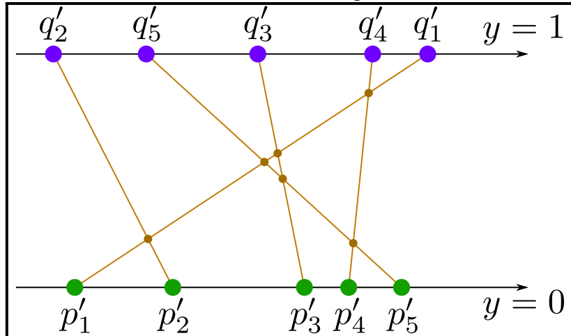
After renaming
