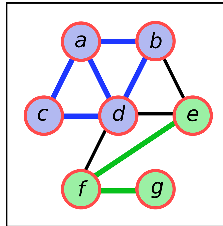
(c) Result computed by our hypergraph algorithms
