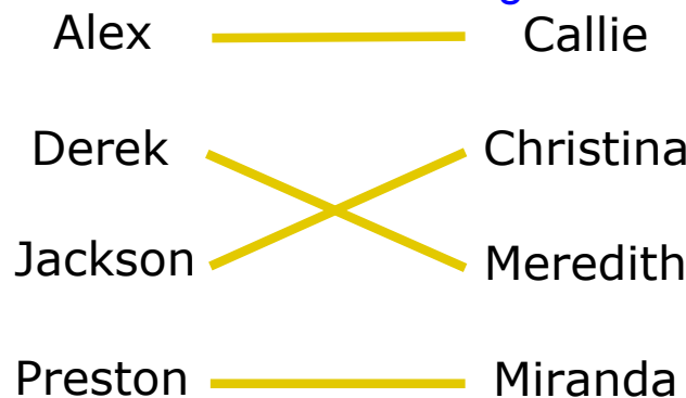
(b) Perfect matching
