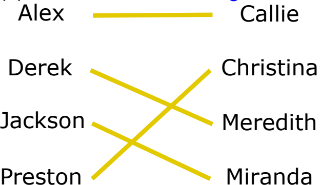
(c) Perfect matching
