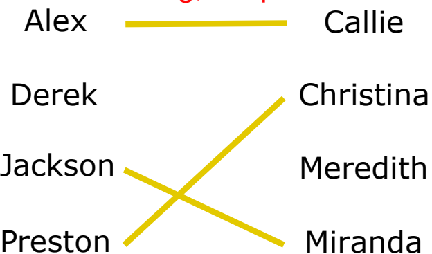
(a) Matching, not perfect
