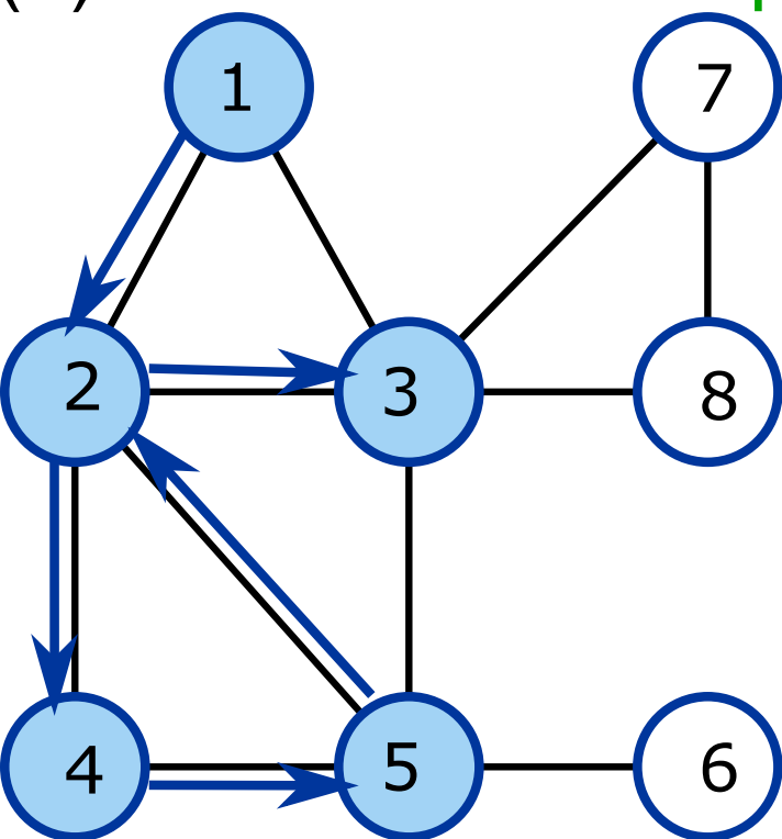
(a) Non-simple path
