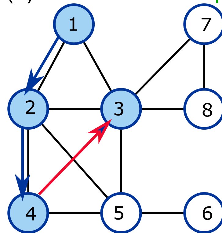
(b) Not a path
