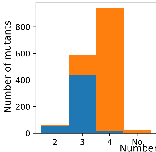
Rescued Mutants
