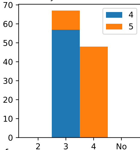
Synthetic Lethals
