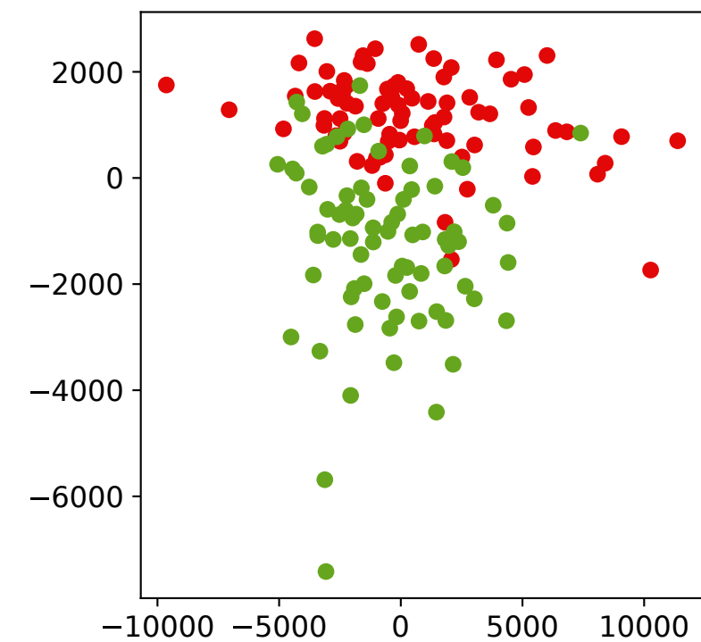
Principal Component 1 (b) PCA on cell cycle related genes
