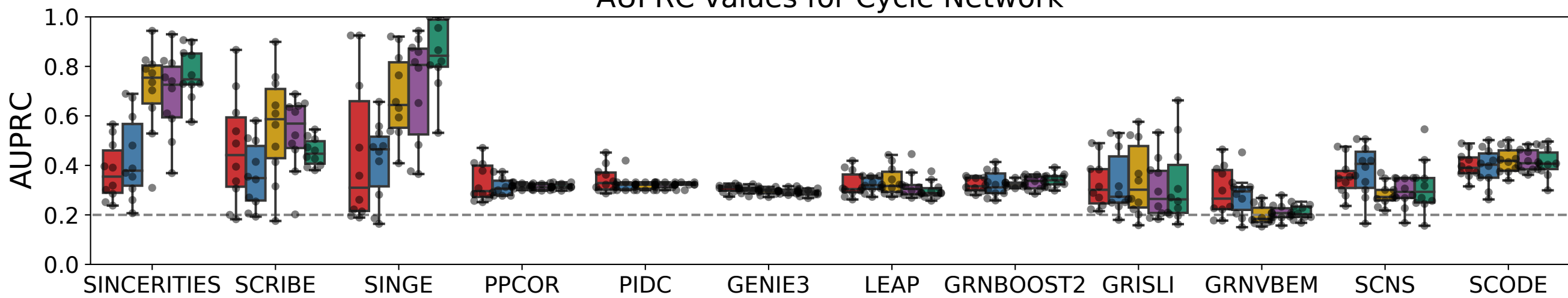
AUPRC values for Cycle Network
