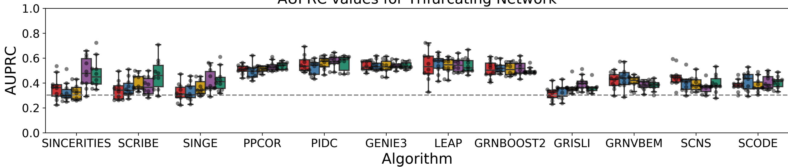
AUPRC values for Trifurcating Network
