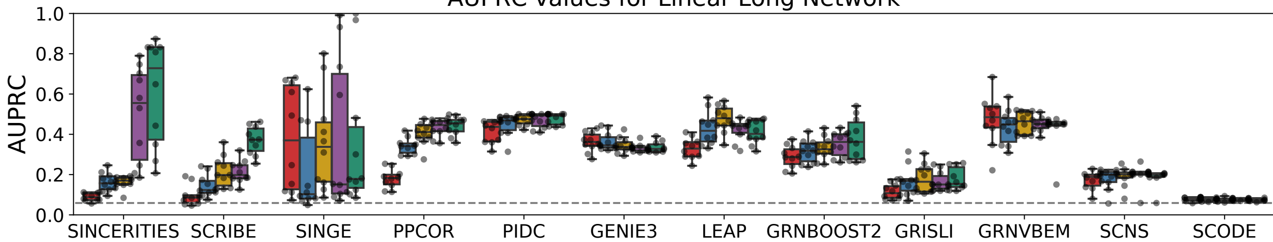
AUPRC values for Linear Long Network
