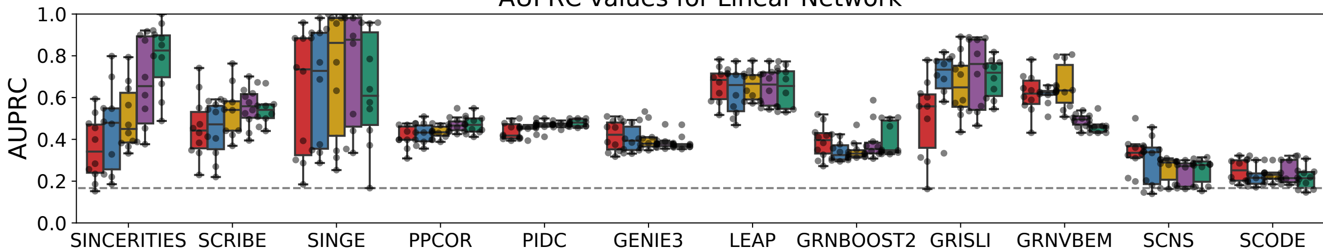
AUPRC values for Linear Network
