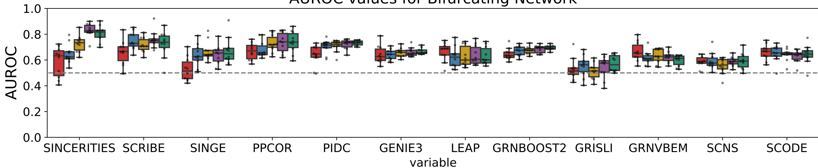
AUROC values for Bifurcating Converging Network
