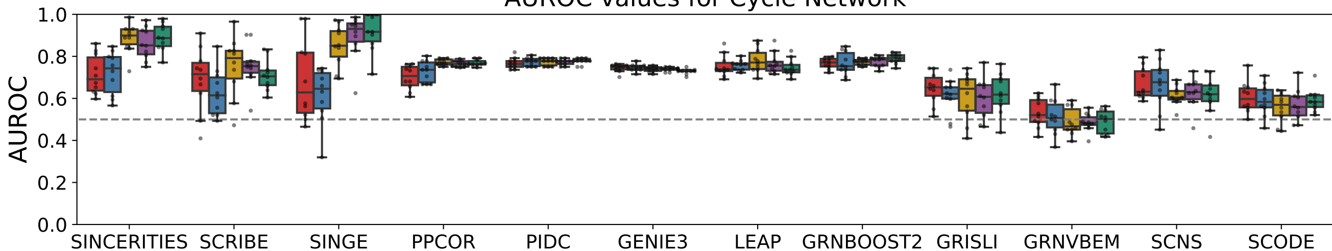
AUROC values for Cycle Network
