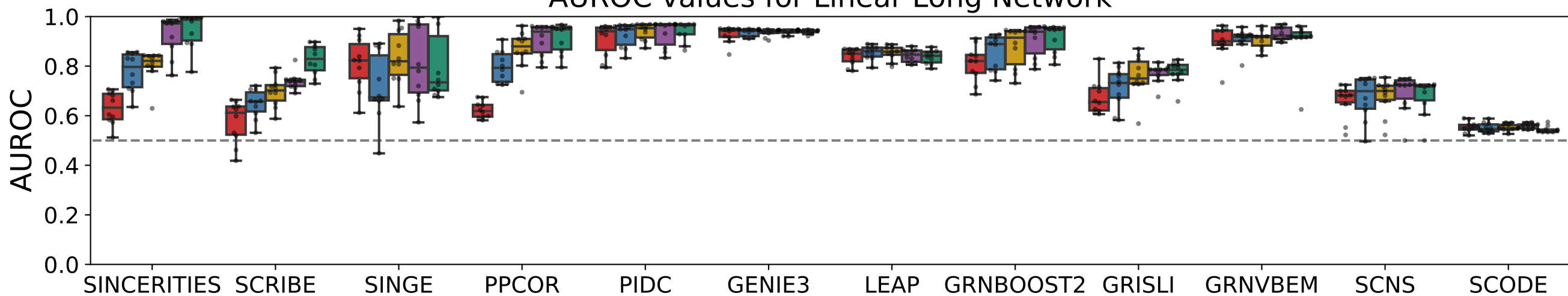
AUROC values for Linear Long Network
