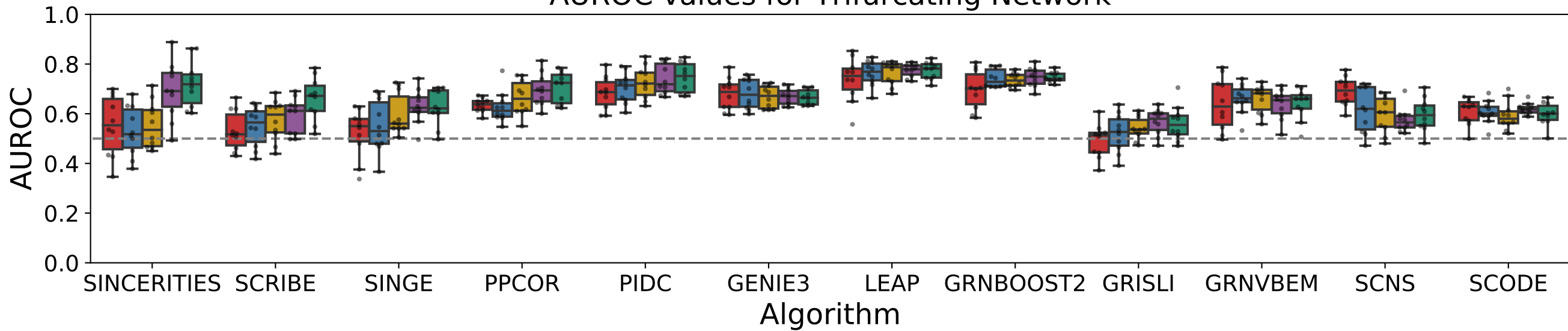
AUROC values for Trifurcating Network
