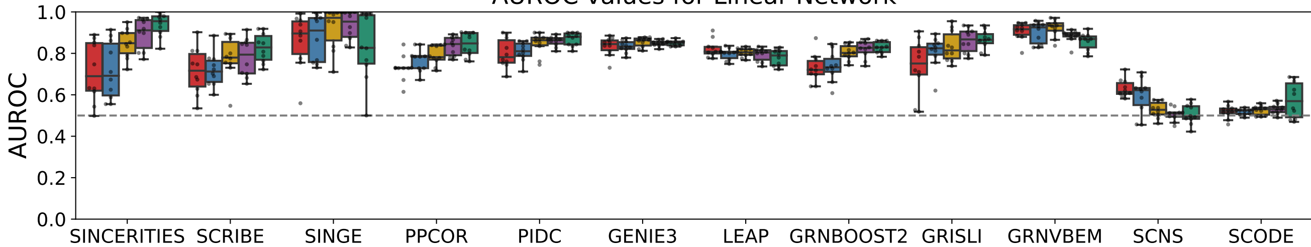
AUROC values for Linear Network
