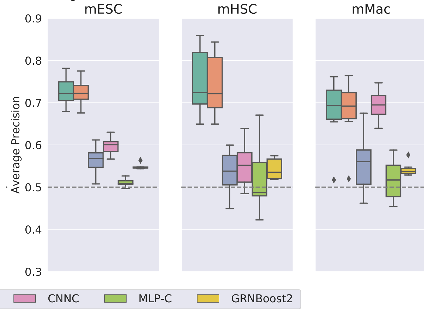
(b) Average Precision
