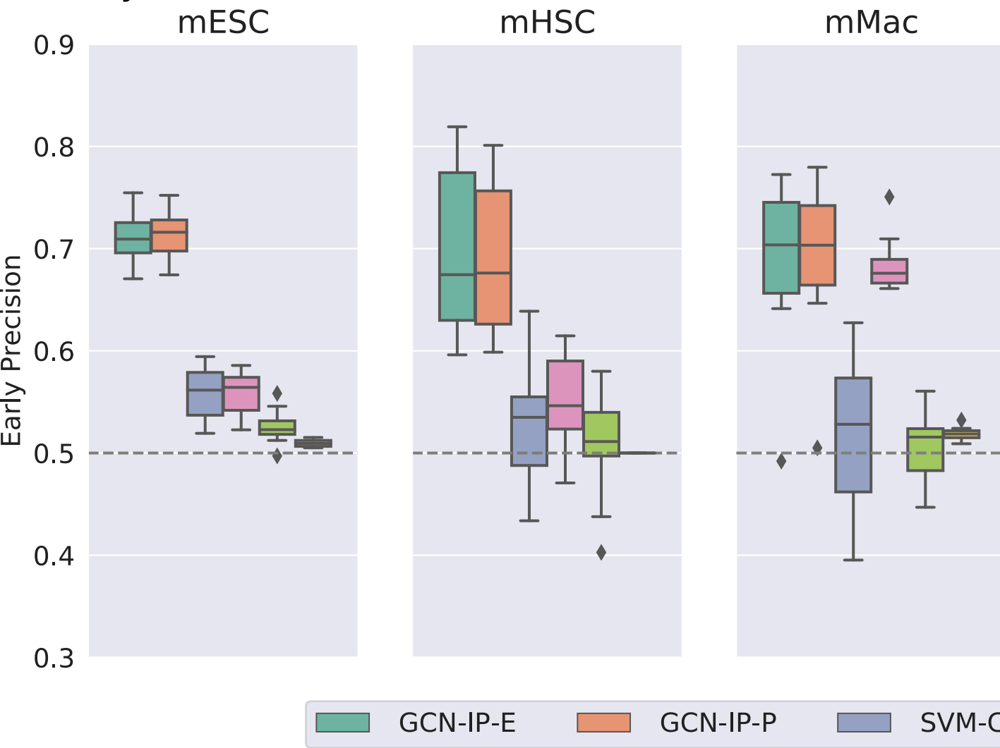
(a) Early Precision
