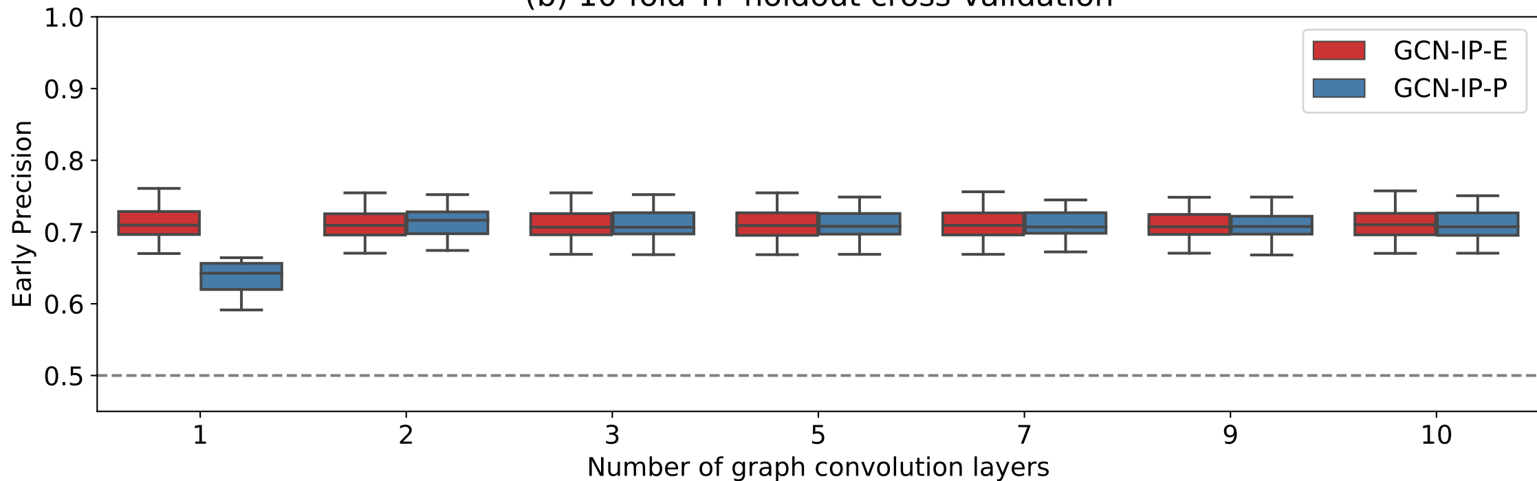
(b) 10-fold TF-holdout cross-validation
