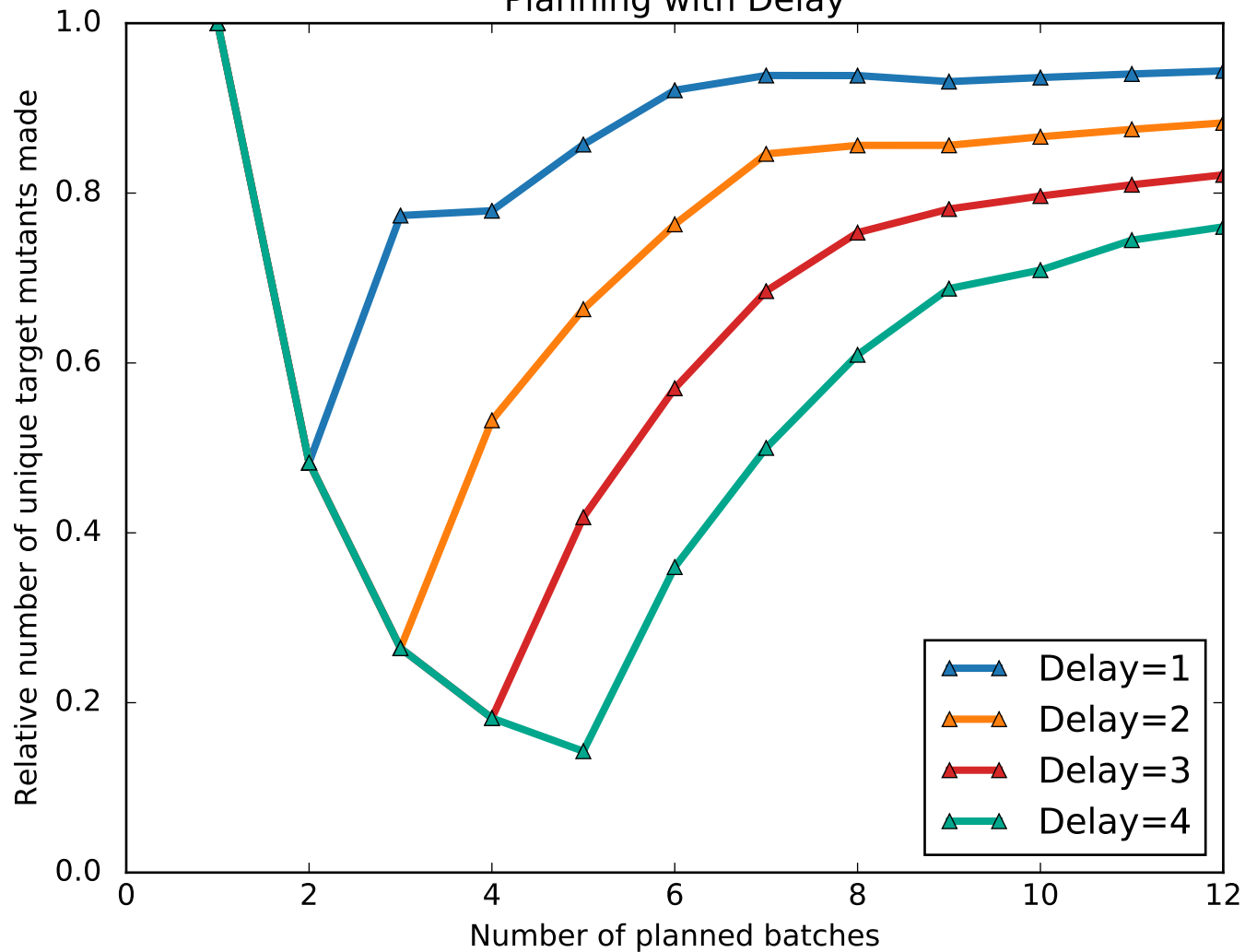
Planning with Delay
