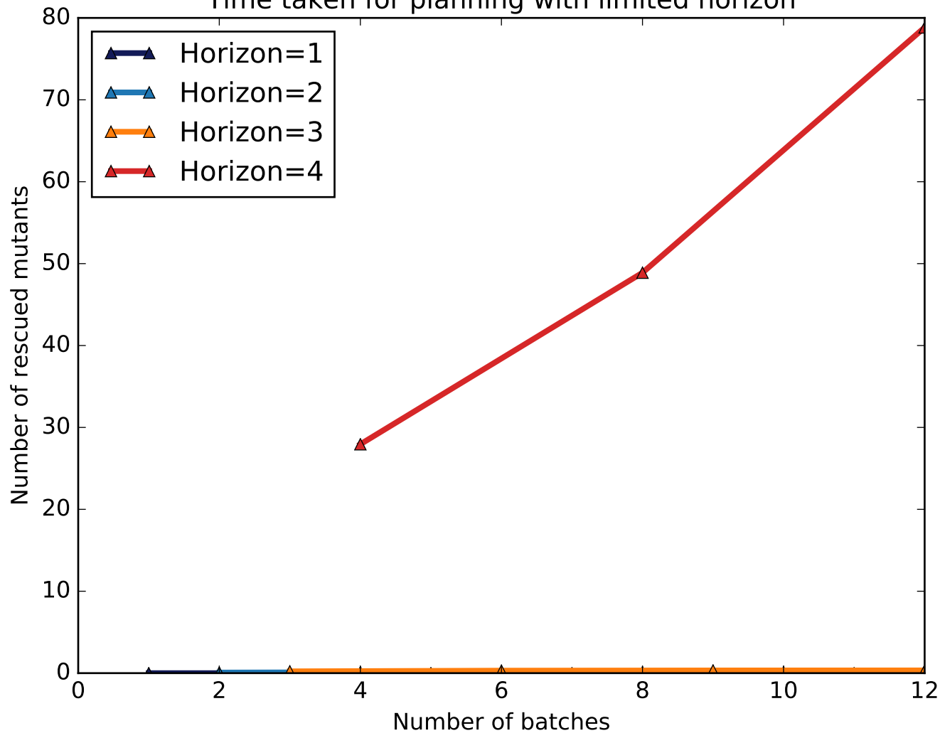
Time taken for planning with limited horizon
