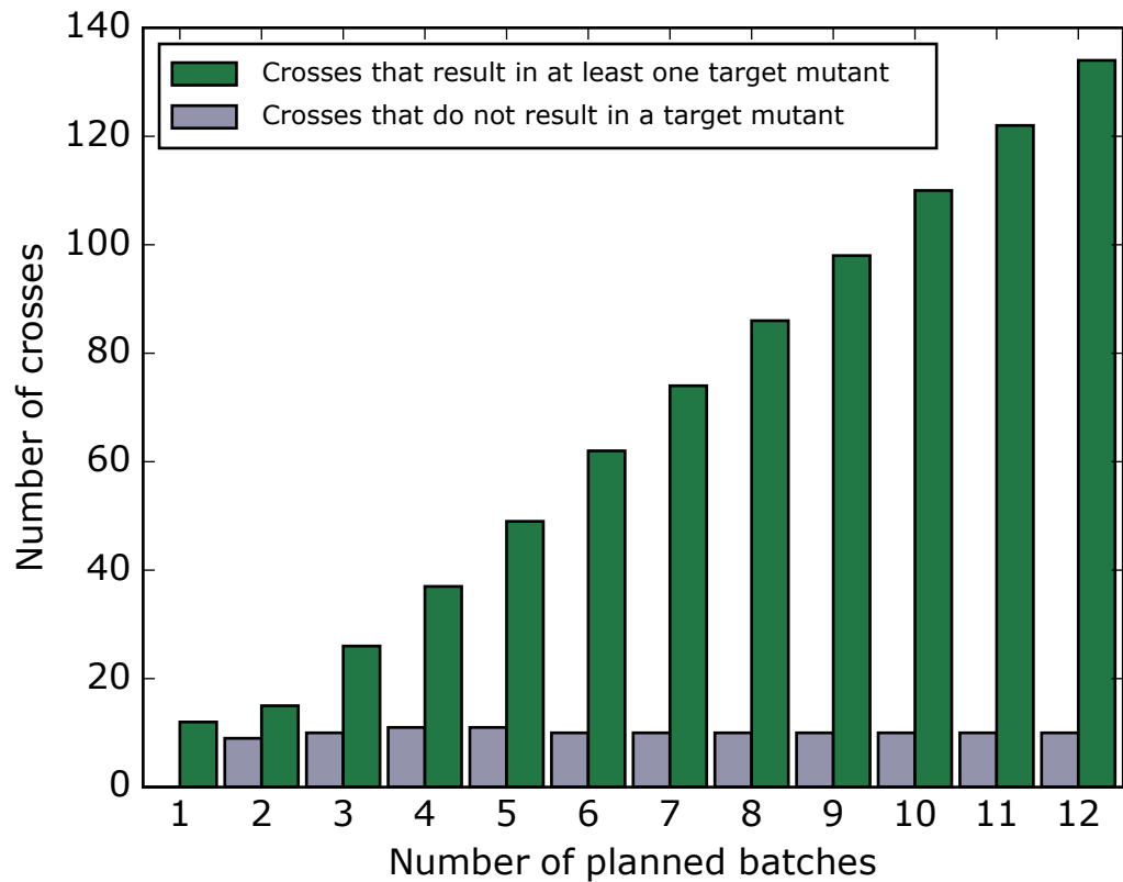
(b) Variation of number of crosses that result in a target mutant with k
