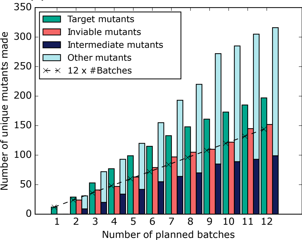
(a) Variation of number of mutants made with k
