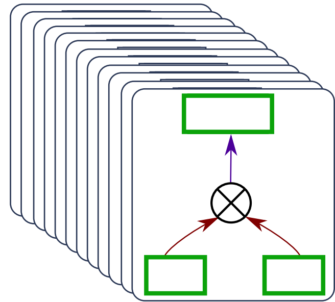
Batch k
