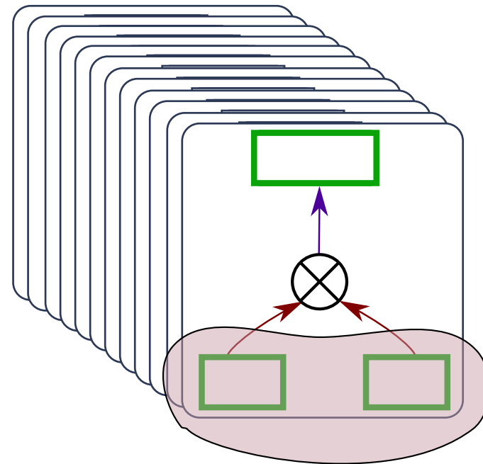
Batch i
