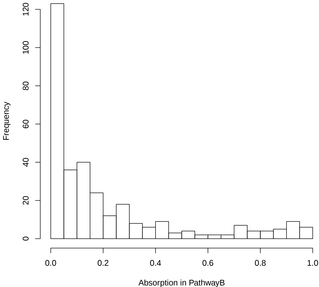
Histogram of absorption in PathwayB (q=0.2)
