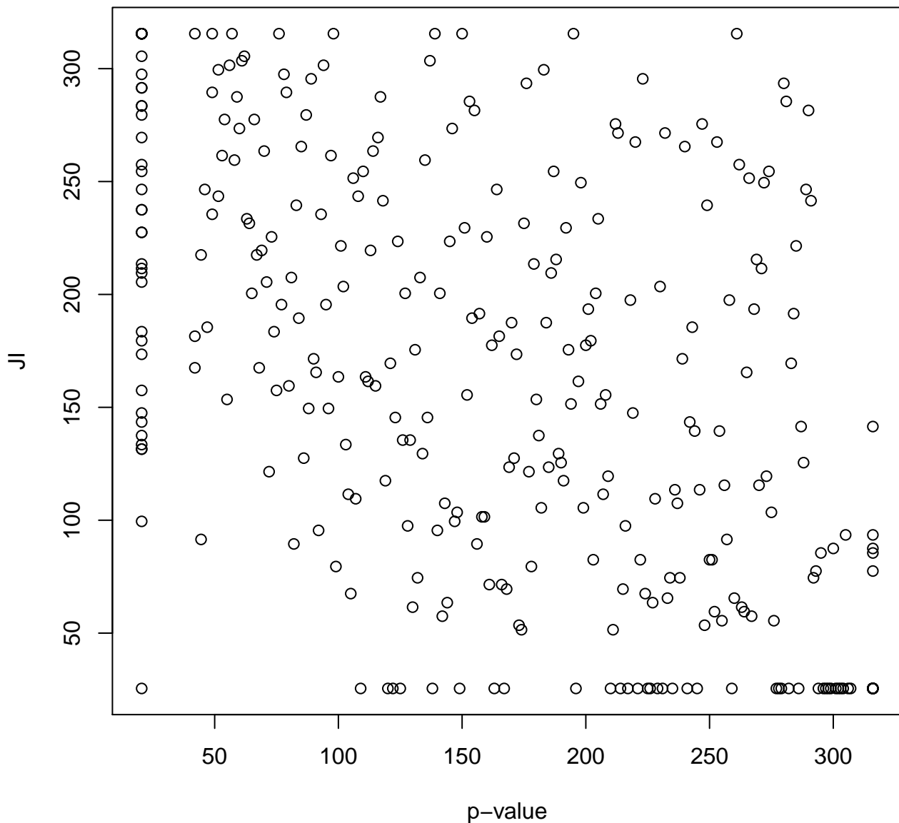
Jaccard Index versus p-value-- Spearman Ranks ( R=-0.220930 )
