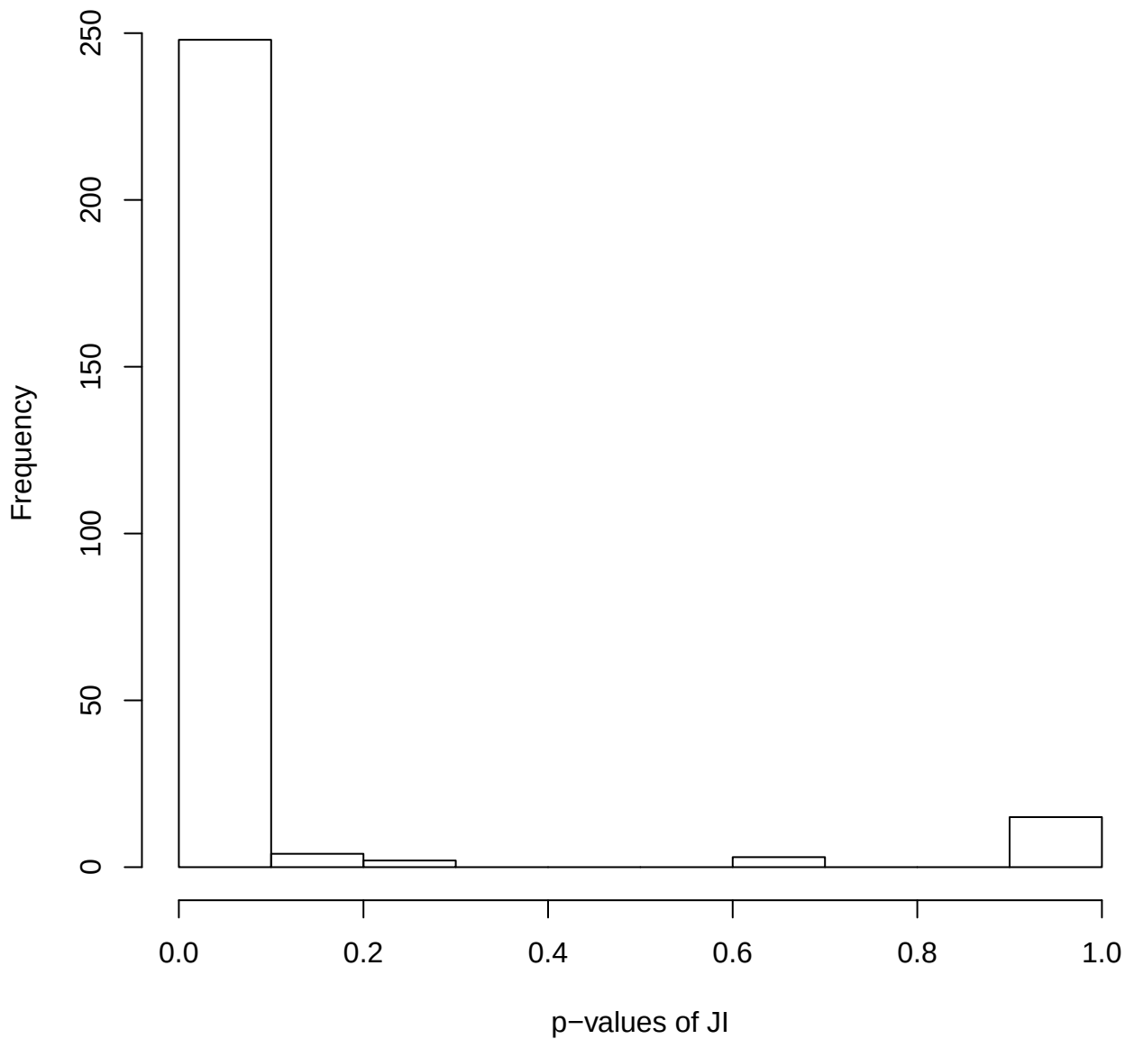
Histogram of p-value for JI between two pathways
