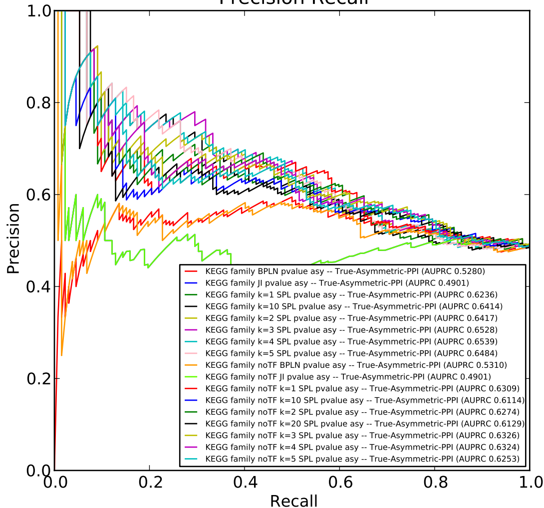
Precision Recall
