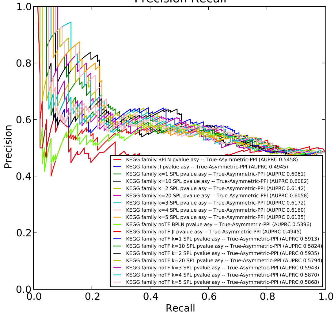
Precision Recall
