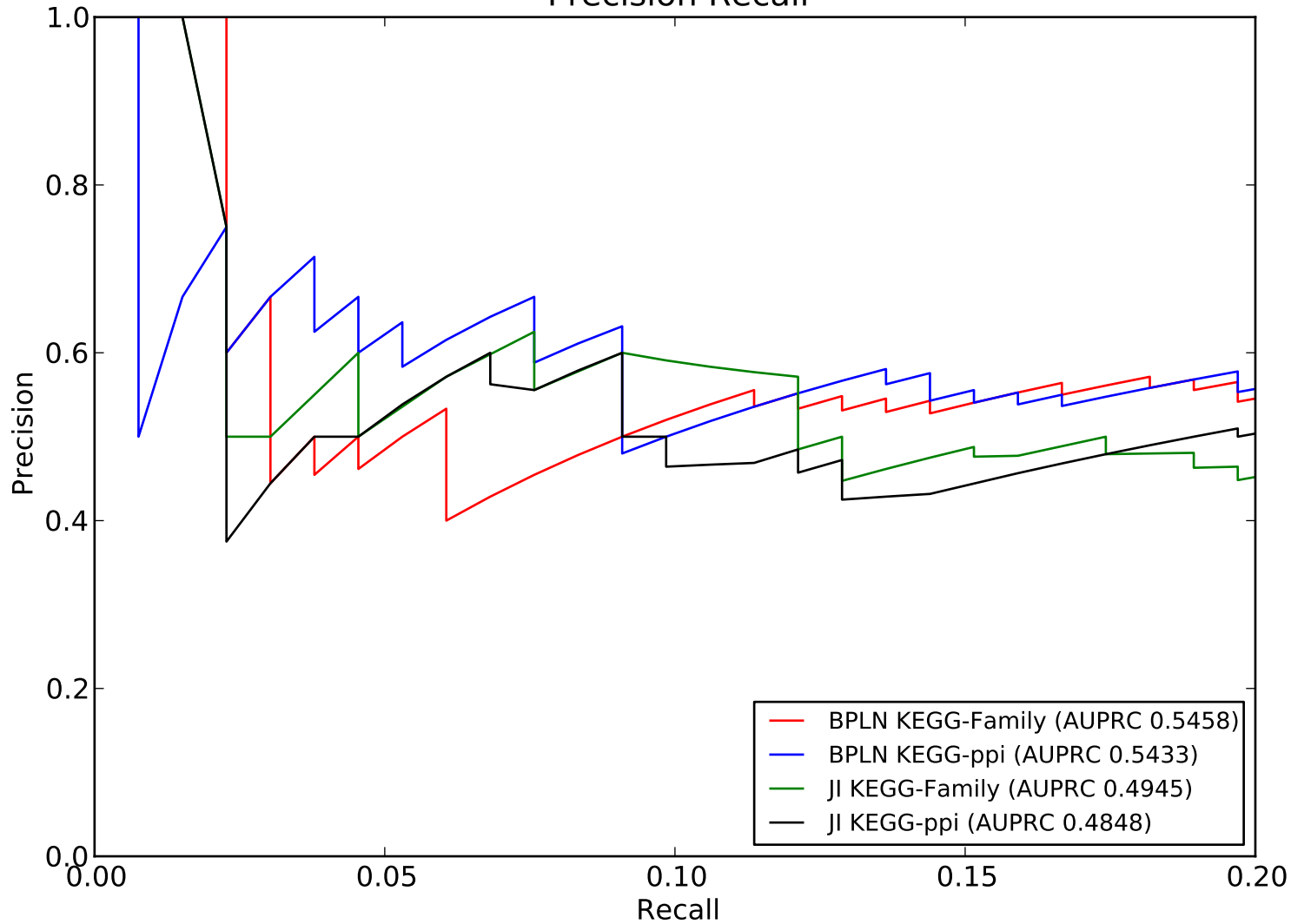
Precision Recall
