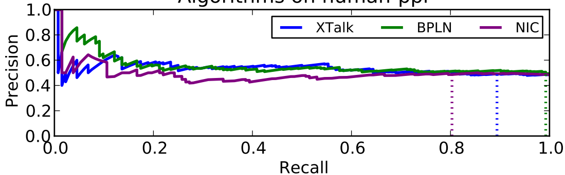
Algorithms on human-ppi
