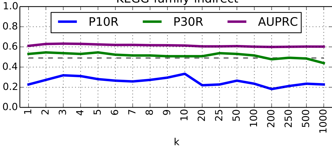
KEGG-family-indirect
