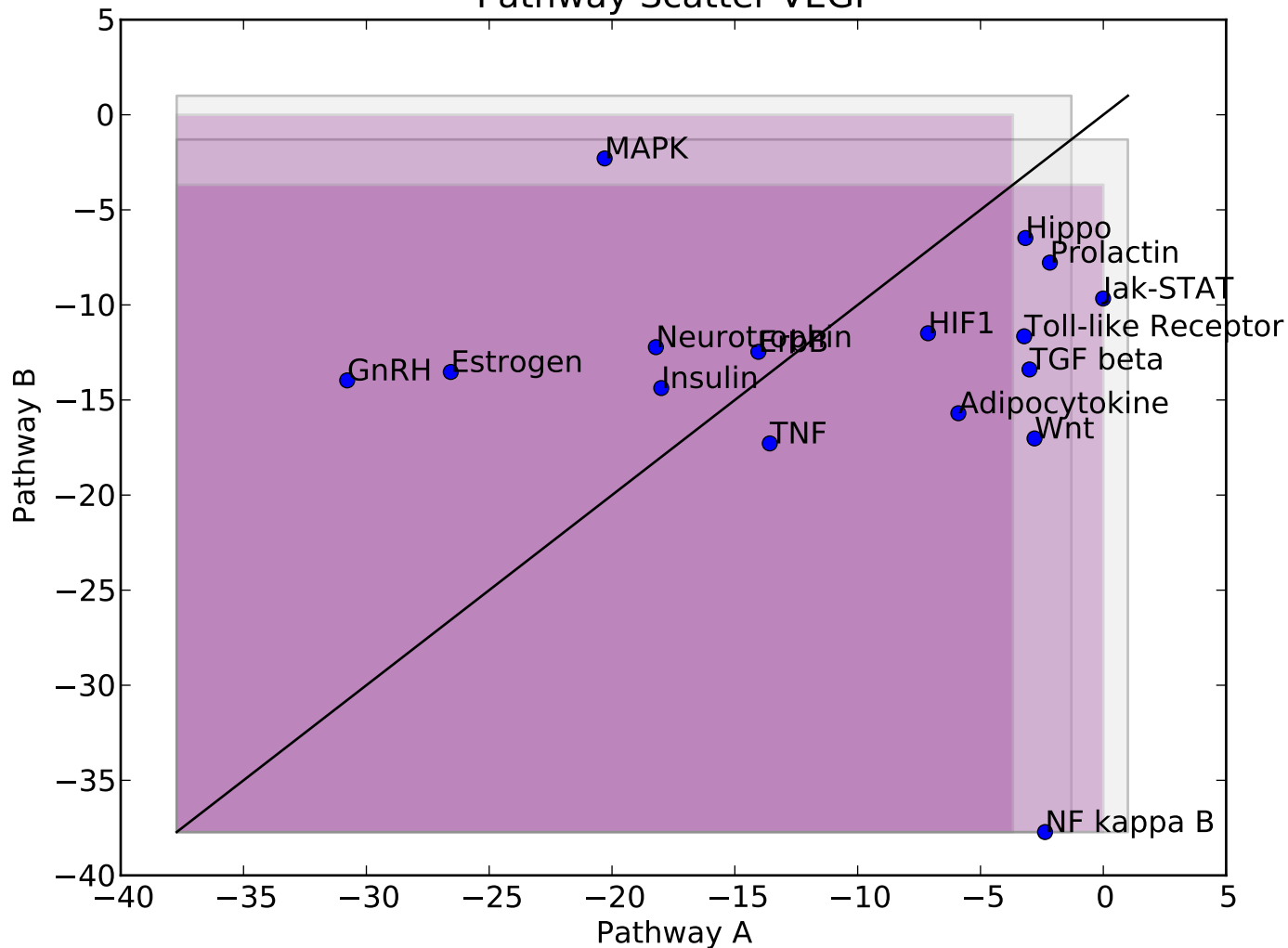
Pathway Scatter VEGF
