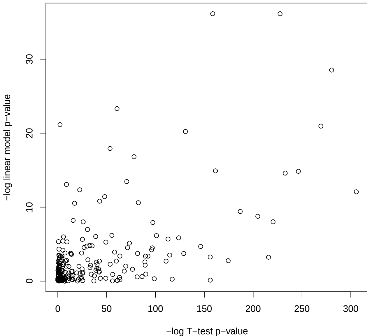
Correlation between T-test and linear model parameter p-values
