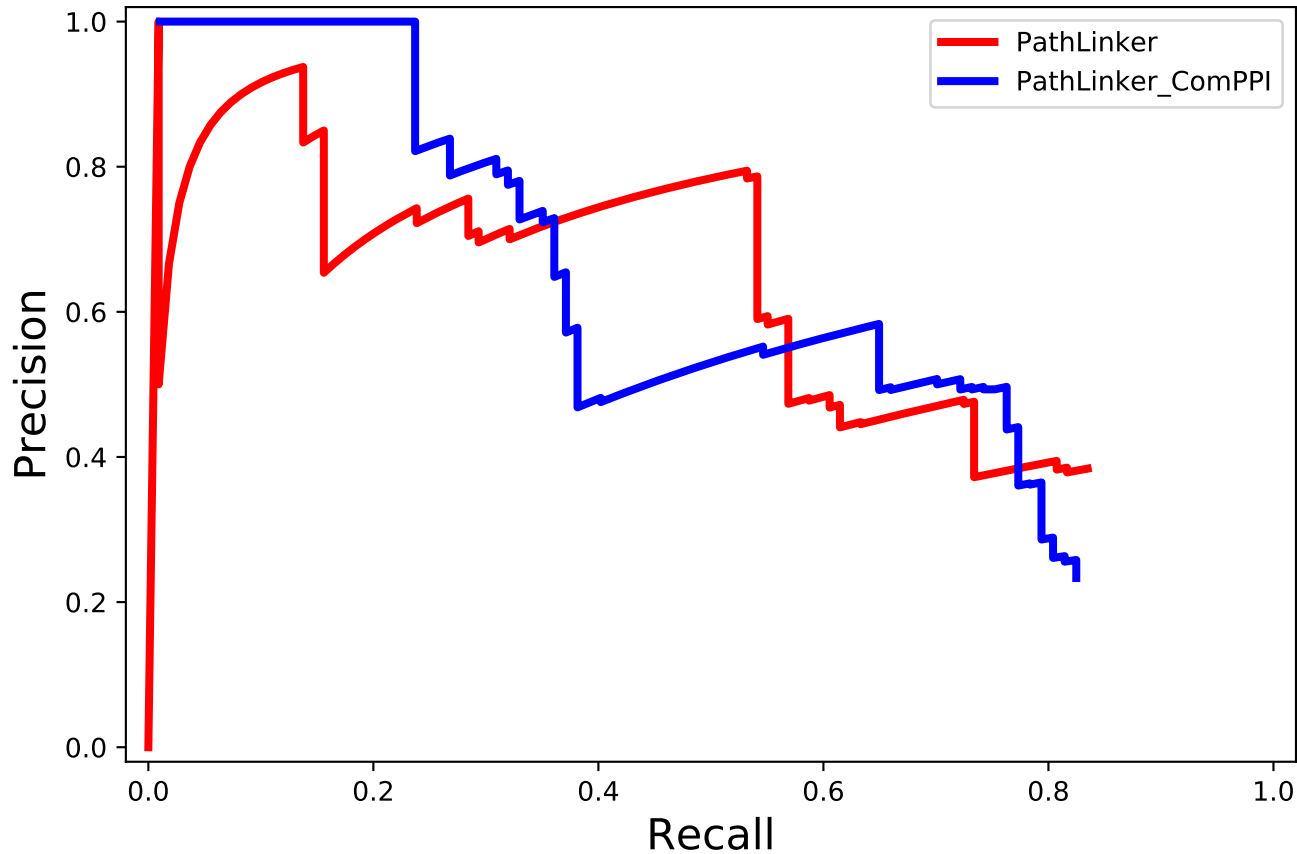
PR Curve
