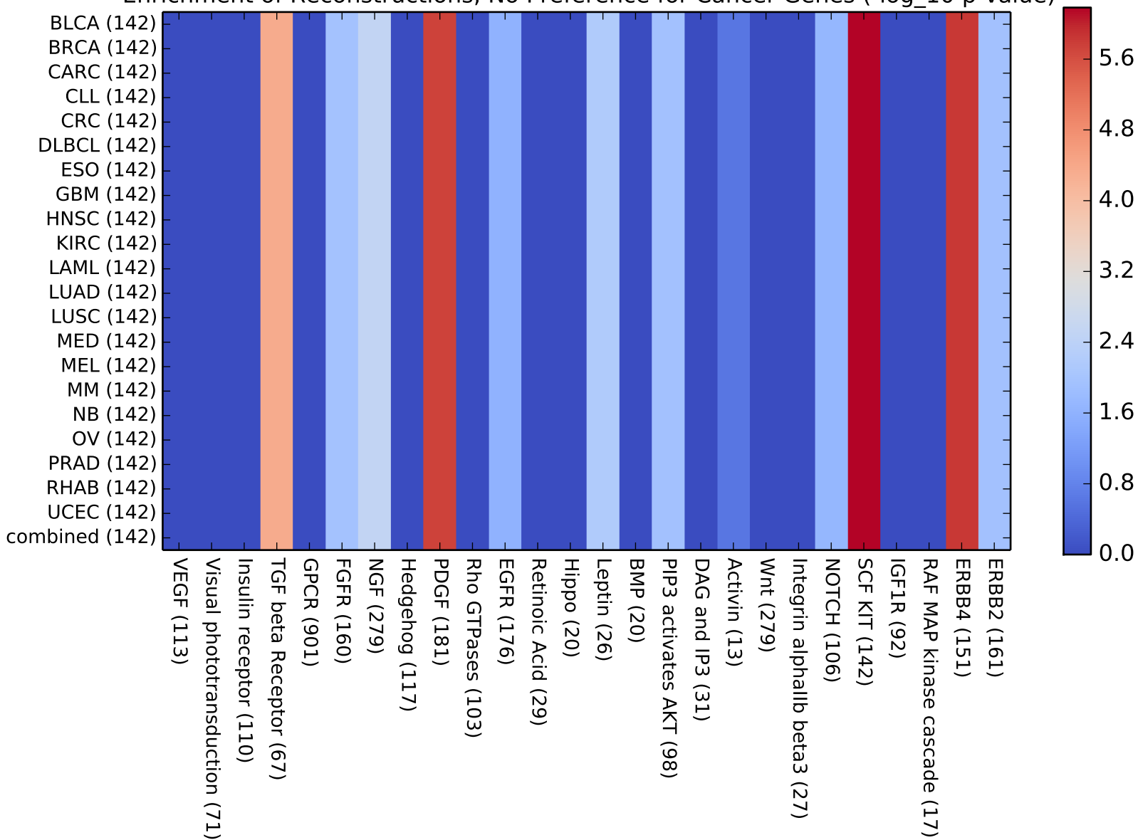
Enrichment of Reconstructions, No Preference for Cancer Genes (-log 10 p-value)
