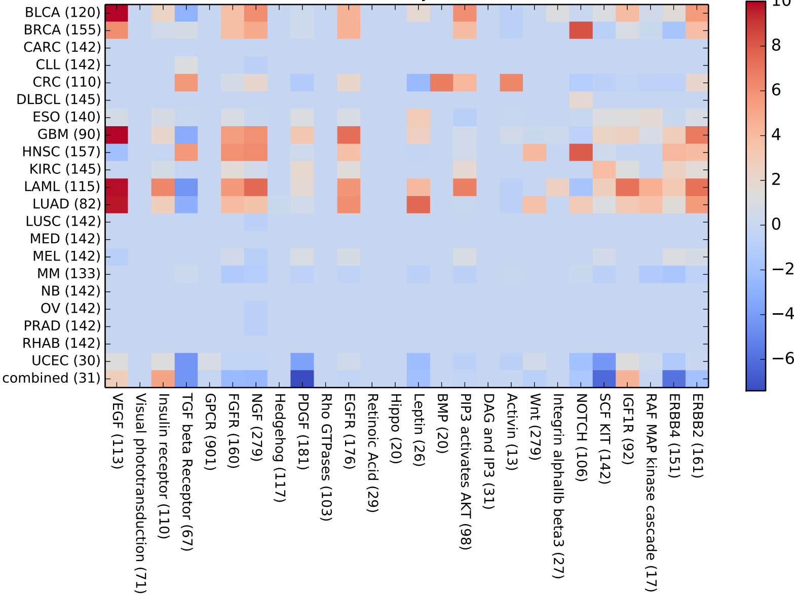
Enrichment of Reconstructions NORMALIZED by Cancer Genes & Unbiased Reconstruction
