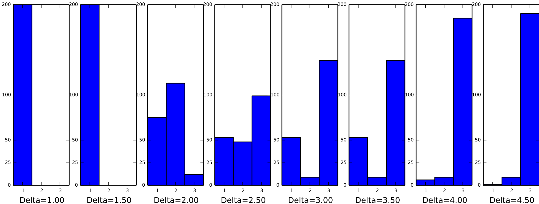
Path length distribution 200 shortest paths on "combined", varying delta
