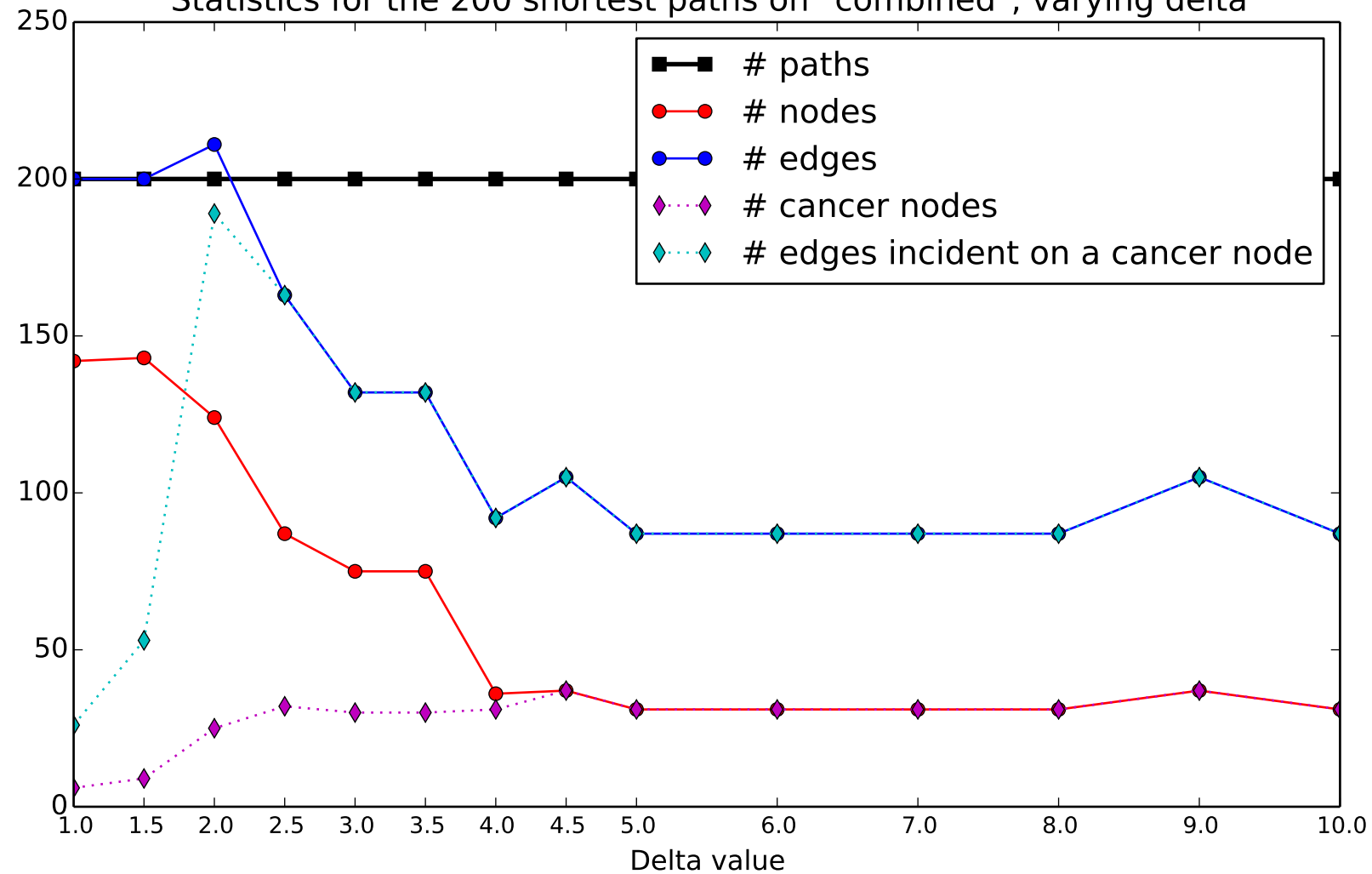
Statistics for the 200 shortest paths on "combined", varying delta
