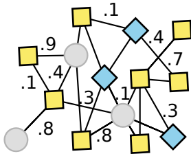
Algorithm Result
