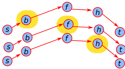
Simple Paths P(s, U, t)
