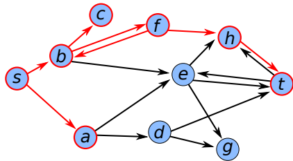
Graph with Complexes
