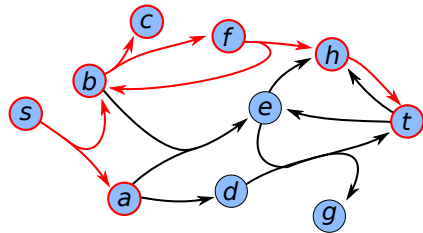
Signaling Hypergraph
