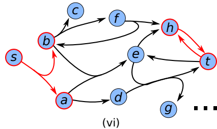
(iv)-(vi): Sub-Hypergraphs that Satisfy ILP Constraints
