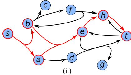
(i)-(iii): s - t B-Hyperpaths of Length 4
