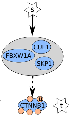
(b) Shortest Path (Graph with Complexes)
