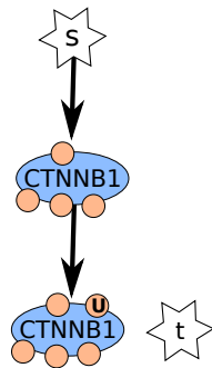
(c) Shortest Path (Graph)
