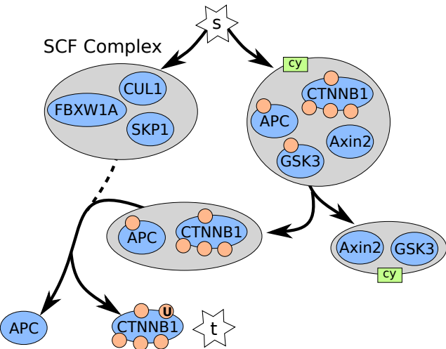
(a) Shortest B-Hyperpath
