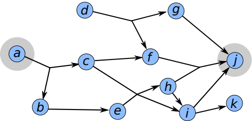
Original Hypergraph
