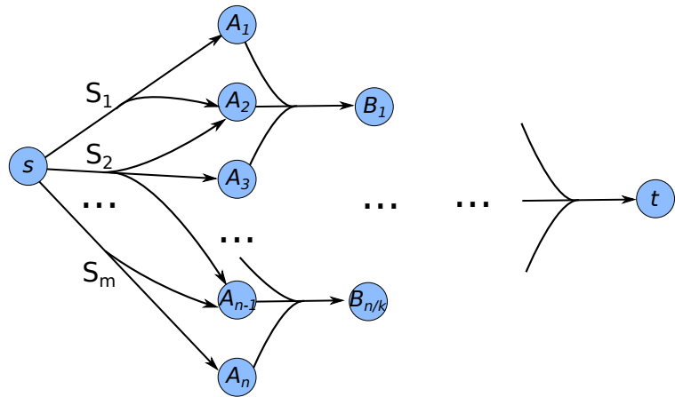
Reduction from Minimum k -Set Cover
