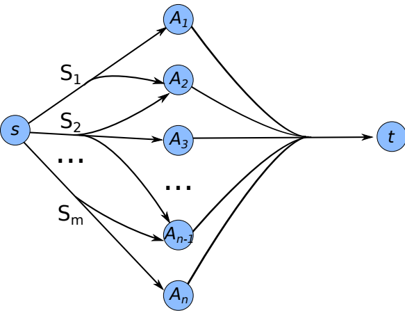
Reduction from Minimum Set Cover
