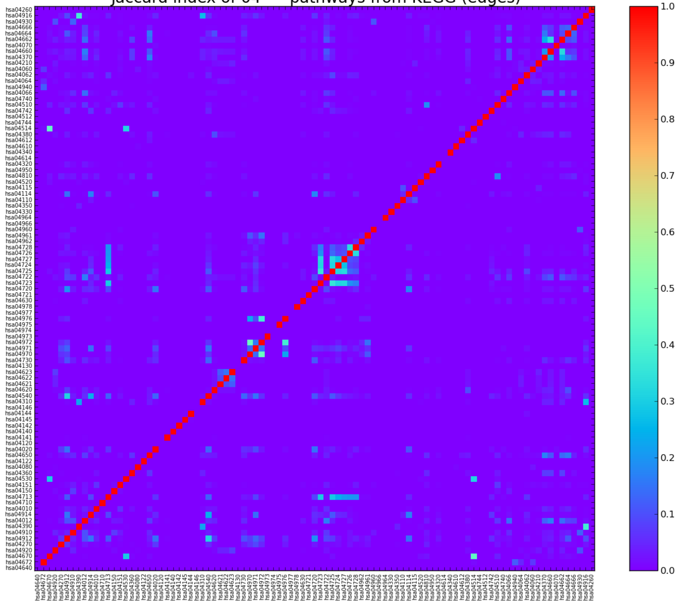
Jaccard index of 04***-pathways from KEGG (edges)
