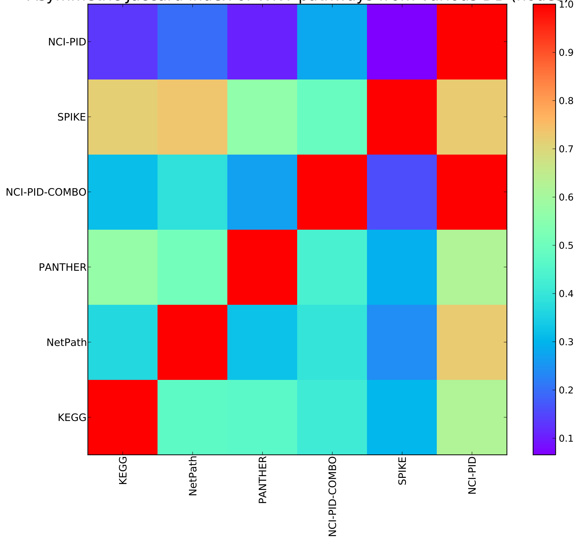
Asymmetric Jaccard index of WNT pathways from various DB (nodes)
