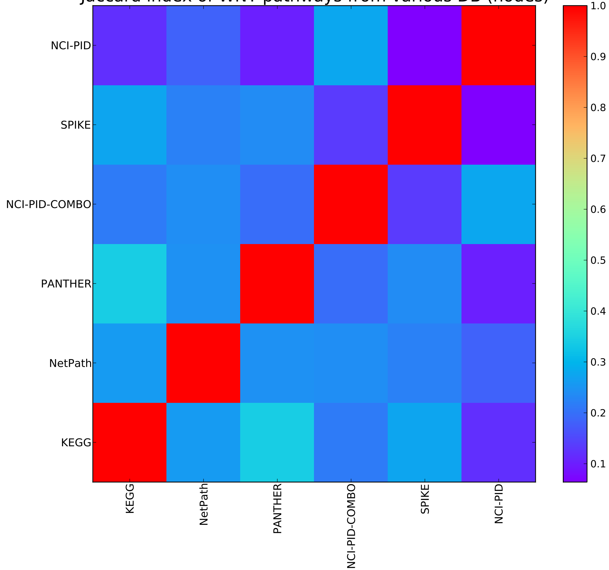
Jaccard index of WNT pathways from various DB (nodes)
