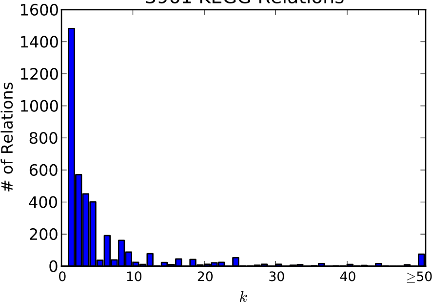
Distribution of 32194 Edges from 3961 KEGG Relations
