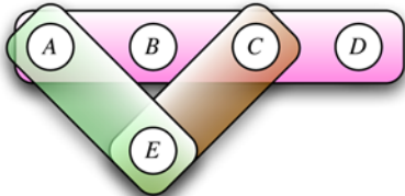
Hypergraph
