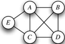
Graph
