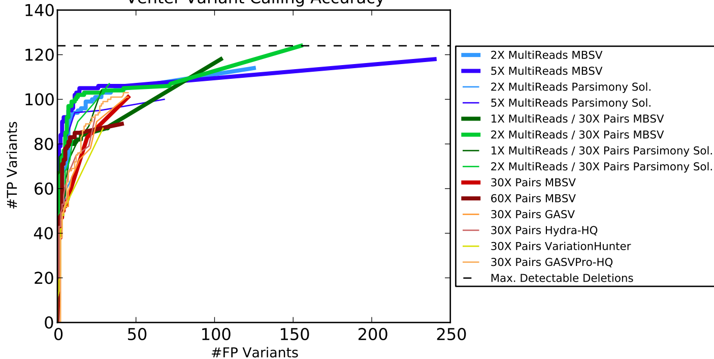
Venter Variant Calling Accuracy
