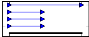
Right Breakpoint
