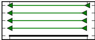
Left Breakpoint
