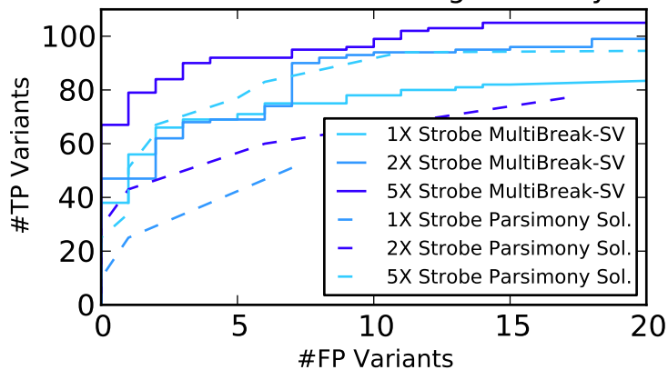
Venter Variant Calling Accuracy
