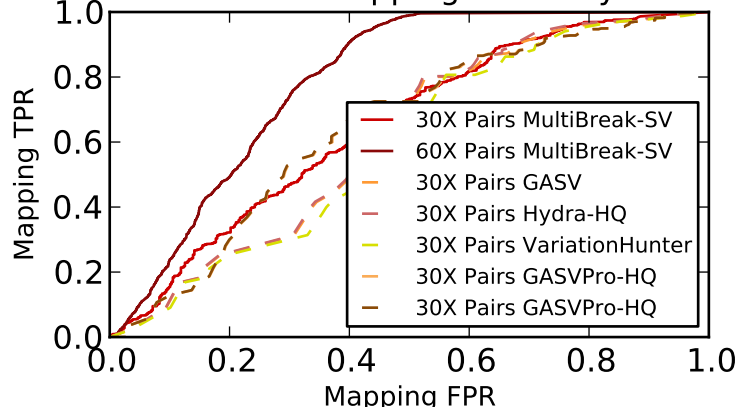
Venter Mapping Accuracy
