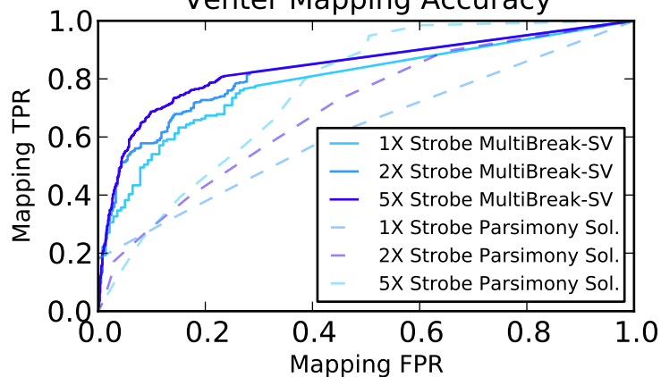
Venter Mapping Accuracy
