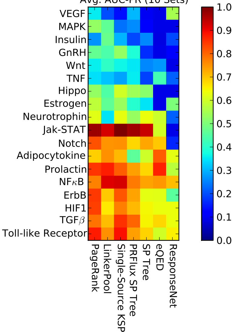
KEGG TFPool Avg. AUC-PR (10 Sets)
