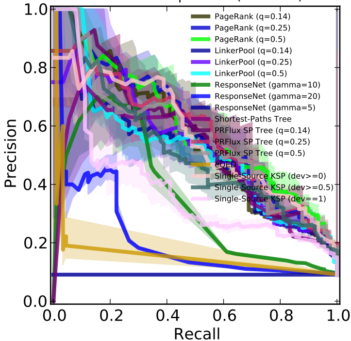
NetPath ReceptorPool (100 Sets)
