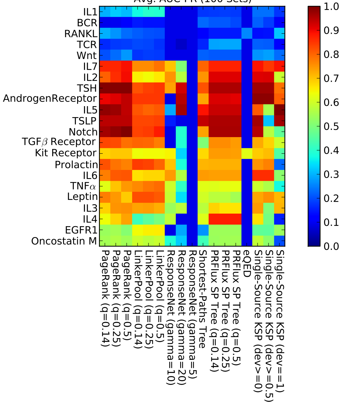
NetPath ReceptorPool Avg. AUC-PR (100 Sets)
